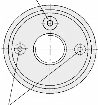
Lock screws
