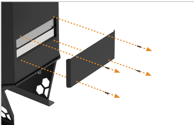
Fig. 16: Removing cover plate for stage 1 & 2 filters
