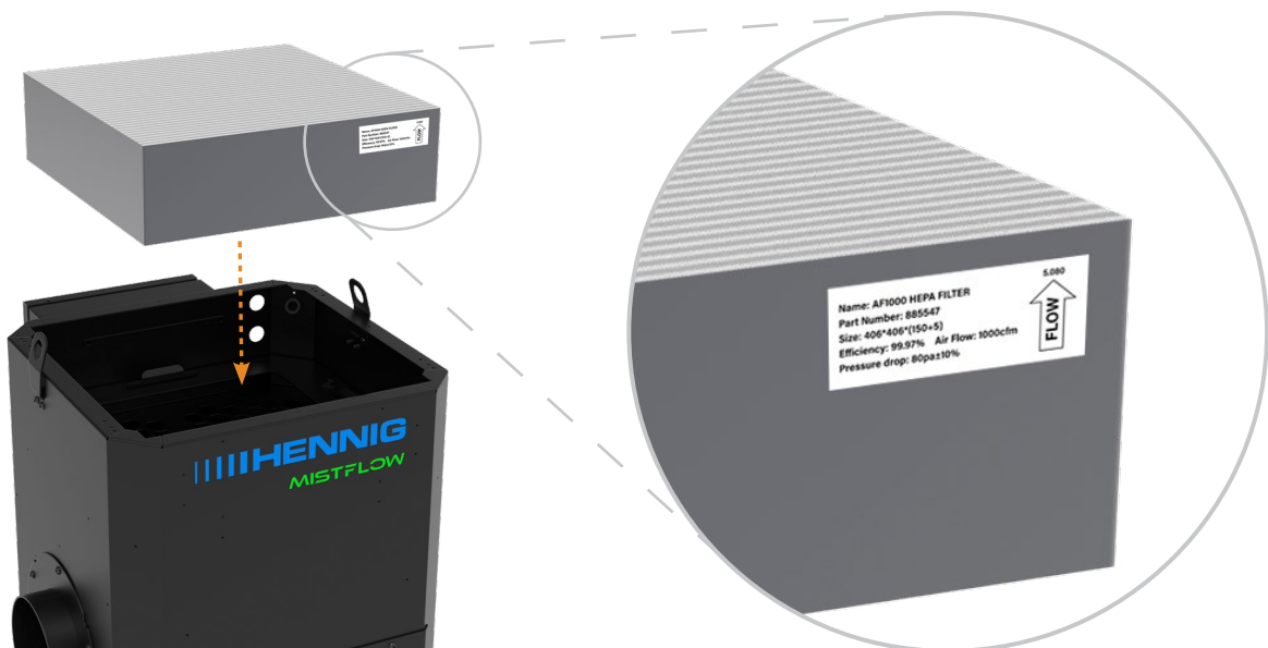
Fig. 20: HEPA filter installation orientation
