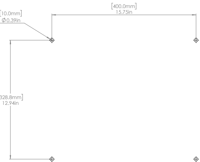
Fig 22: Universal mount bolt pattern
