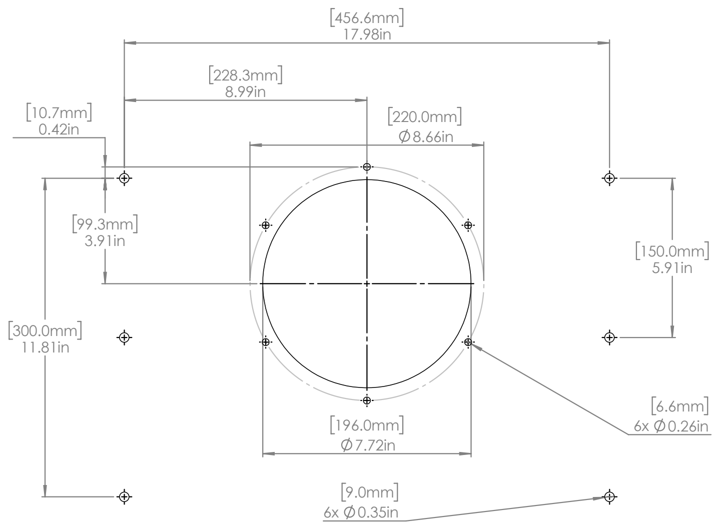
Fig 24: Side mount and hose flange bolt pattern
