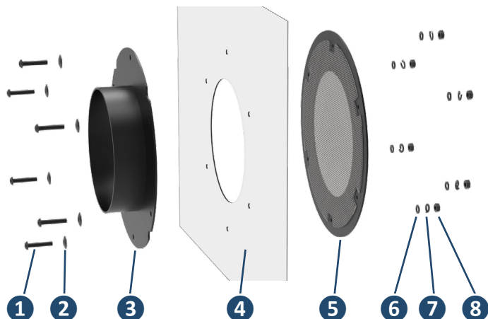
Fig. 1: Installing the hose flange on the machine tool
