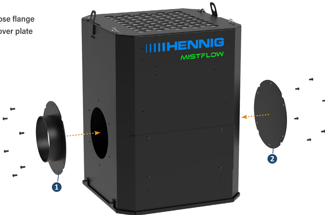
Fig. 2: Installing the hose flange and cover plate on the MistFlow (depending on your application, the hose flange and cover plate could switch sides)
