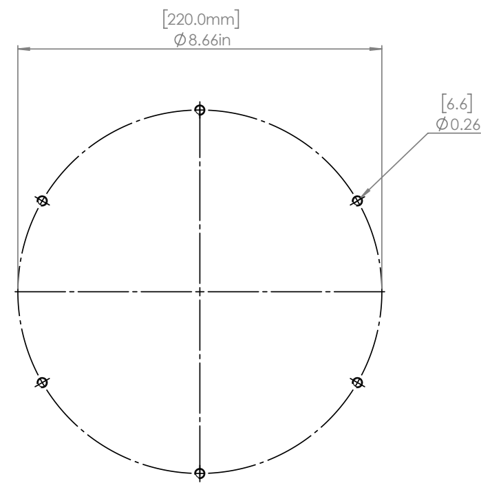
Fig 21: Hose flange bolt pattern Note: The hose flange bolt pattern is the same for the 6" or 8" hose flange plate
