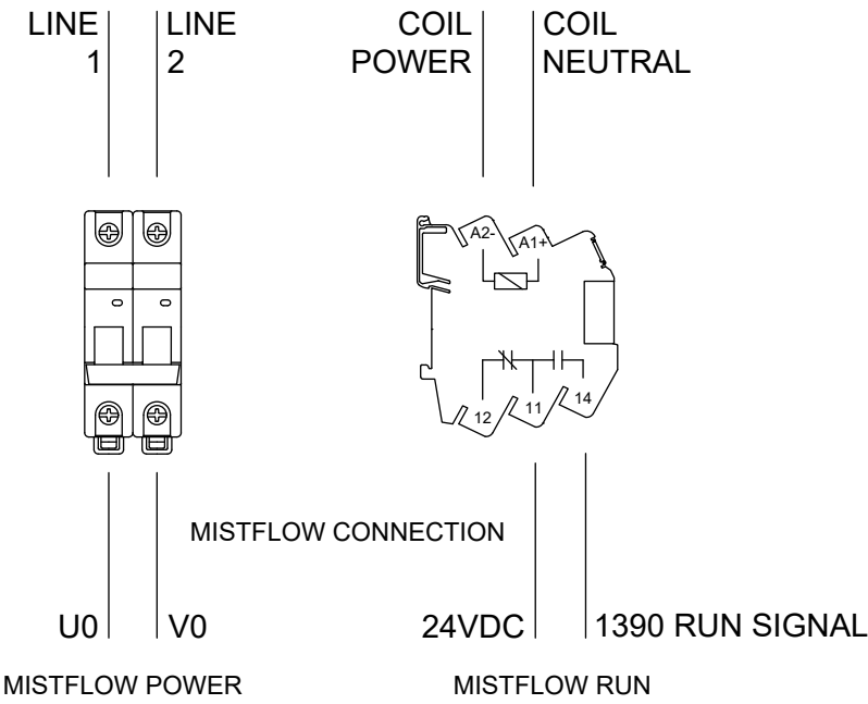
Fig. 15: 230V Power and run signal wiring
