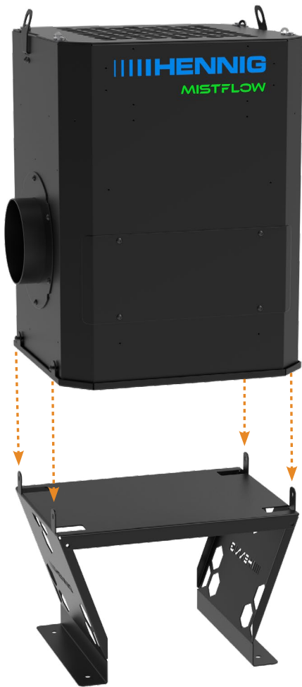
Fig. 3: Placing MistFlow on stand (shown with universal stand)
