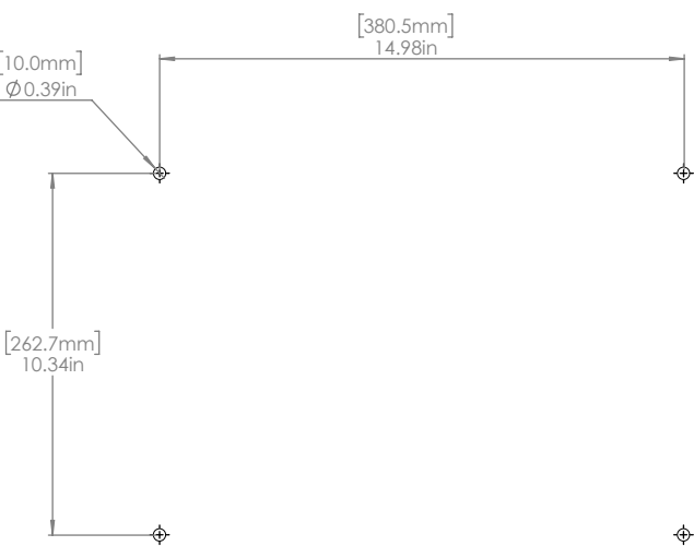
Fig 23: Floor mount bolt pattern
