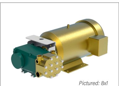
PUMP OPTIONS • 16 x 1 Single 16 GPM piston pump • 8 x 1 Single 8 GPM piston pump • 8 x 2 Dual 8 GPM piston pumps
